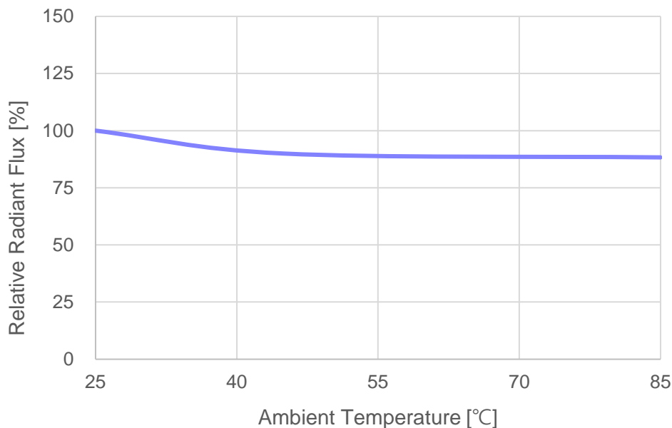
< Ambient Temperature vs. Relative Radiant flux >
